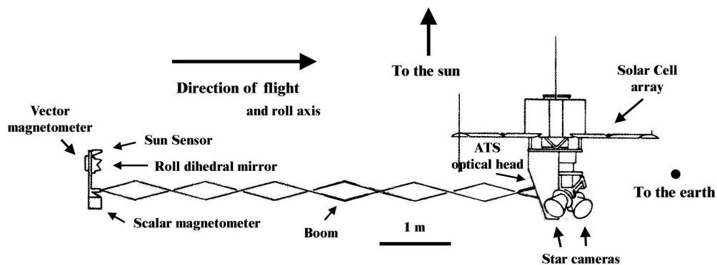
Figure 1. Line drawing of Magsat, its orientation, and critical systems. The roll axis is along the orbital velocity vector, the yaw axis is vertical, and the pitch axis completes the orthogonal coordinate system.
